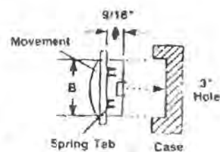
CLOSED ASSEMBLY
