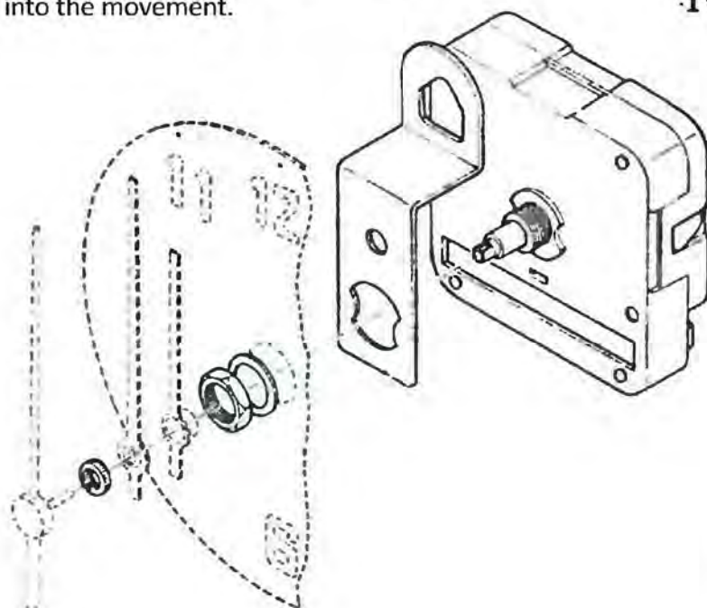
Code: QMXL Extra Long Shaft
